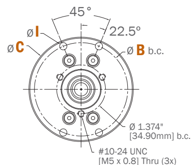
HOUSING FLANGE MOUNT (F1)
