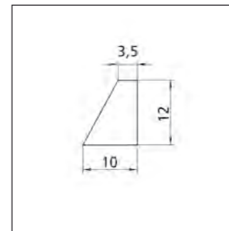
Depth: 130 mm Profile No. 2.3.2.010.012
