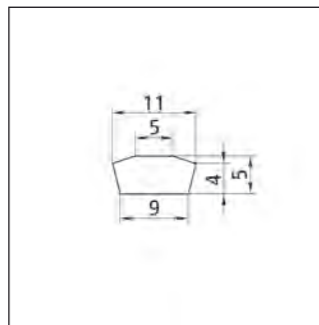
Depth: 25,4 mm Profile No. 2.3.3.011.005
