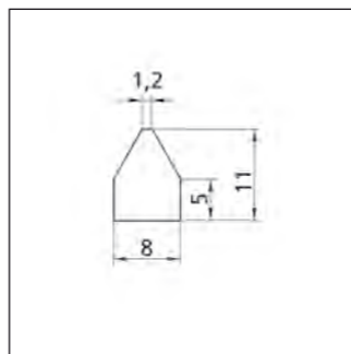
Depth: 10 mm Profile No. 2.3.3.008.011
