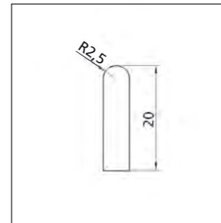
Depth: 100 mm Profile No. 2.3.2.020.005
