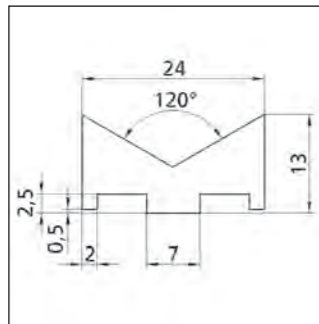
Depth: 15 mm Profile No. 2.3.3.013.024
