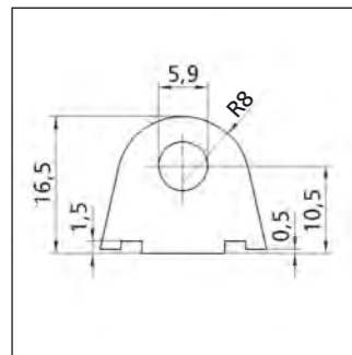
Depth: 15 mm Profile No. 2.3.3.016.020
