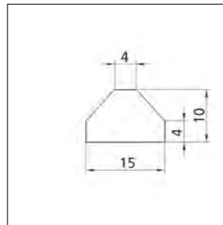
Depth: 35 mm Profile No. 2.3.3.015.010
