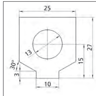
Depth: 50 mm Profile No. 2.3.2.025.027
