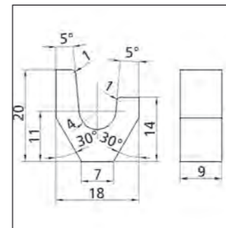
Profile No. 2.3.2.018.020
