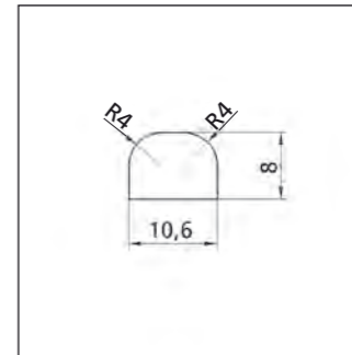
Depth: 100 mm Profile No. 2.3.2.008.010
