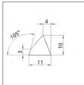
Depth: 98 mm Profile No. 2.3.3.011.010
