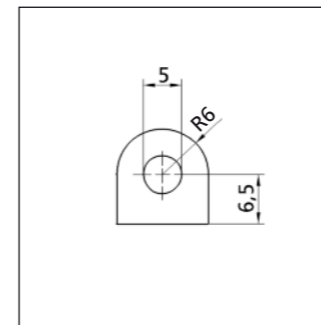
Depth: 50 mm Profile No. 2.3.2.012.012
