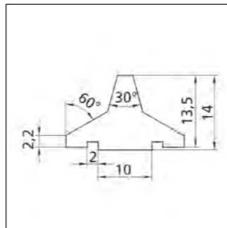
Depth: 170 mm Profile No. 2.3.3.014.022
