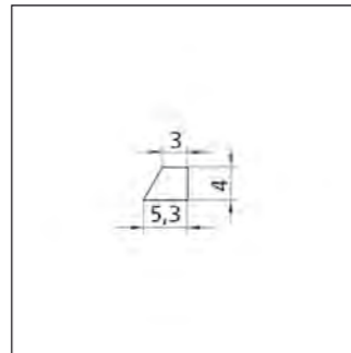
Depth: 25 mm Profile No. 2.3.3.004.005
