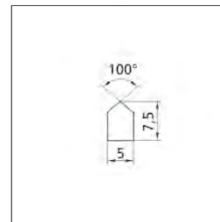
Depth: 100 mm Profile No. 2.3.2.005.007
