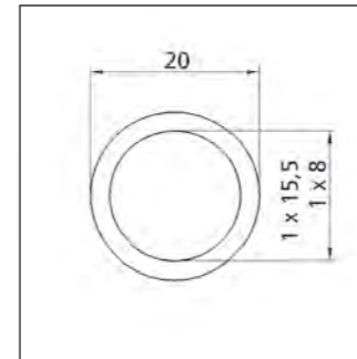
Depth: 50 mm Profile No. 2.3.1.015.020
