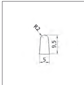
Depth: free Profile No. 2.3.3.009.005
