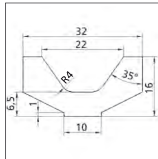
Depth: 15 mm Profile No. 2.3.3.016.032
