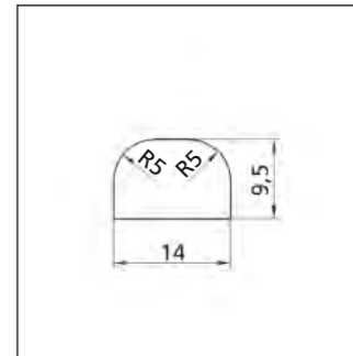
Depth: 64 and 100 mm Profile No. 2.3.2.009.014
