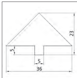
Depth: 100 mm Profile No. 2.3.3.023.036
